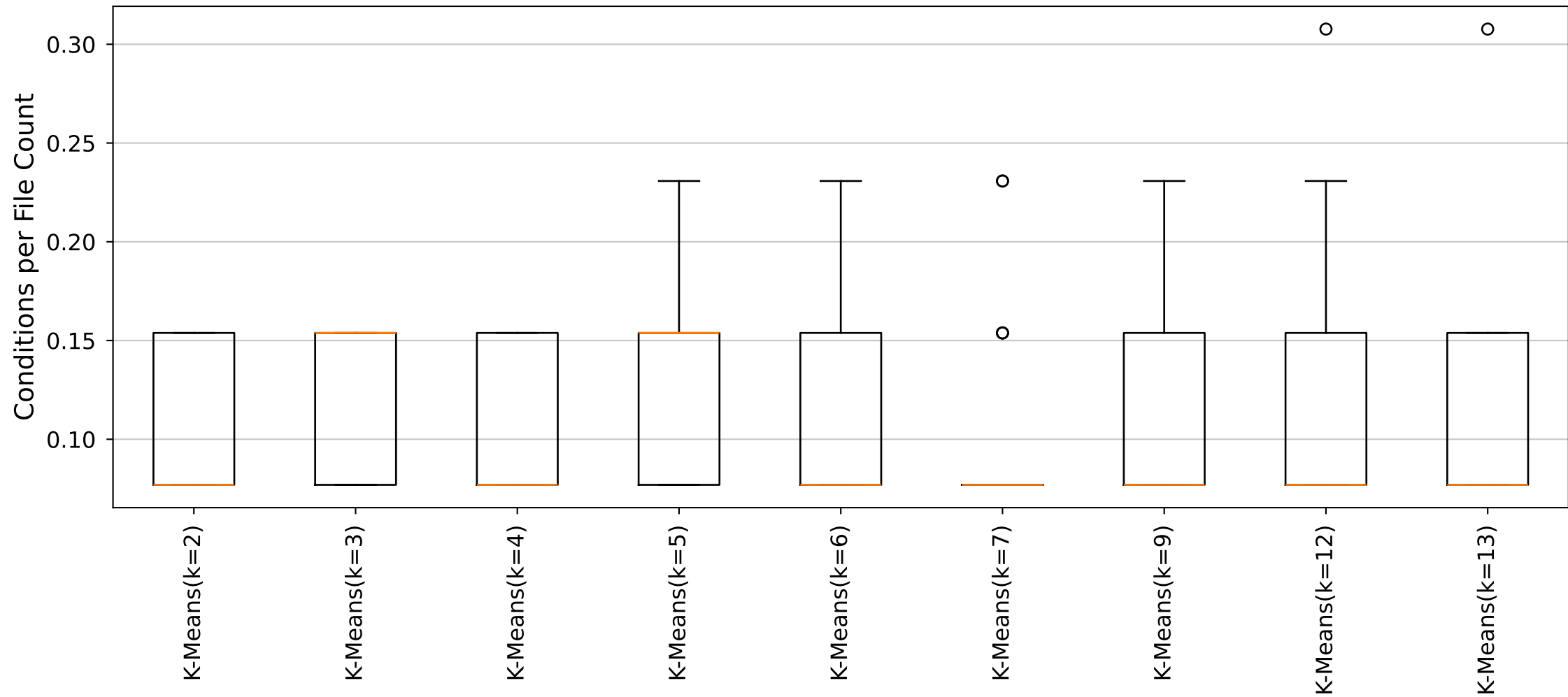
YARA Rules Conditions per File Count Distribution (Cluster8_Size13 dataset)
